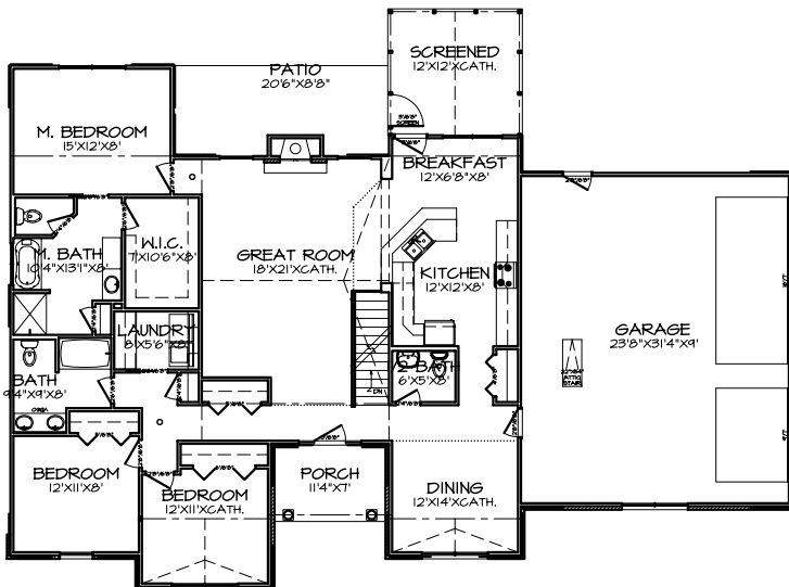
1 FIRST FLOOR PLAN A-4
